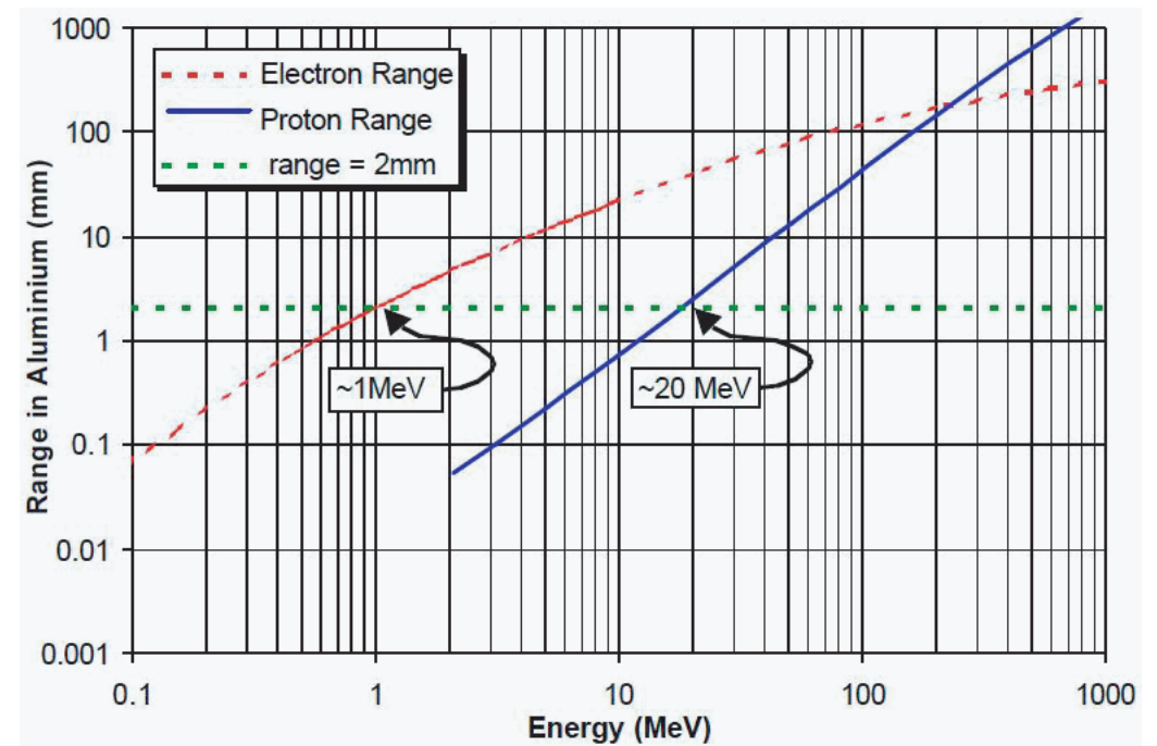
Fig.5.5: Ranges of electron and proton in aluminum. With about 3mm aluminum, CCD can be shielded from the proton of 25MeV.
