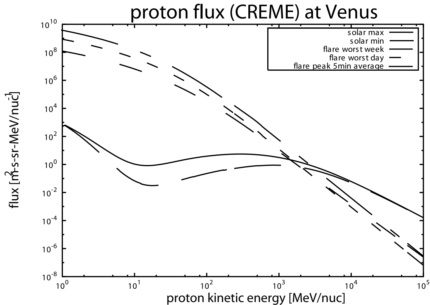
Fig.5.4: The proton flux around Venus which is estimated using the CREME model. At the time of a flare event, it is monotonous reduction as it becomes high energy. At the time of quiet time, it has an extremum near GeV energy.
