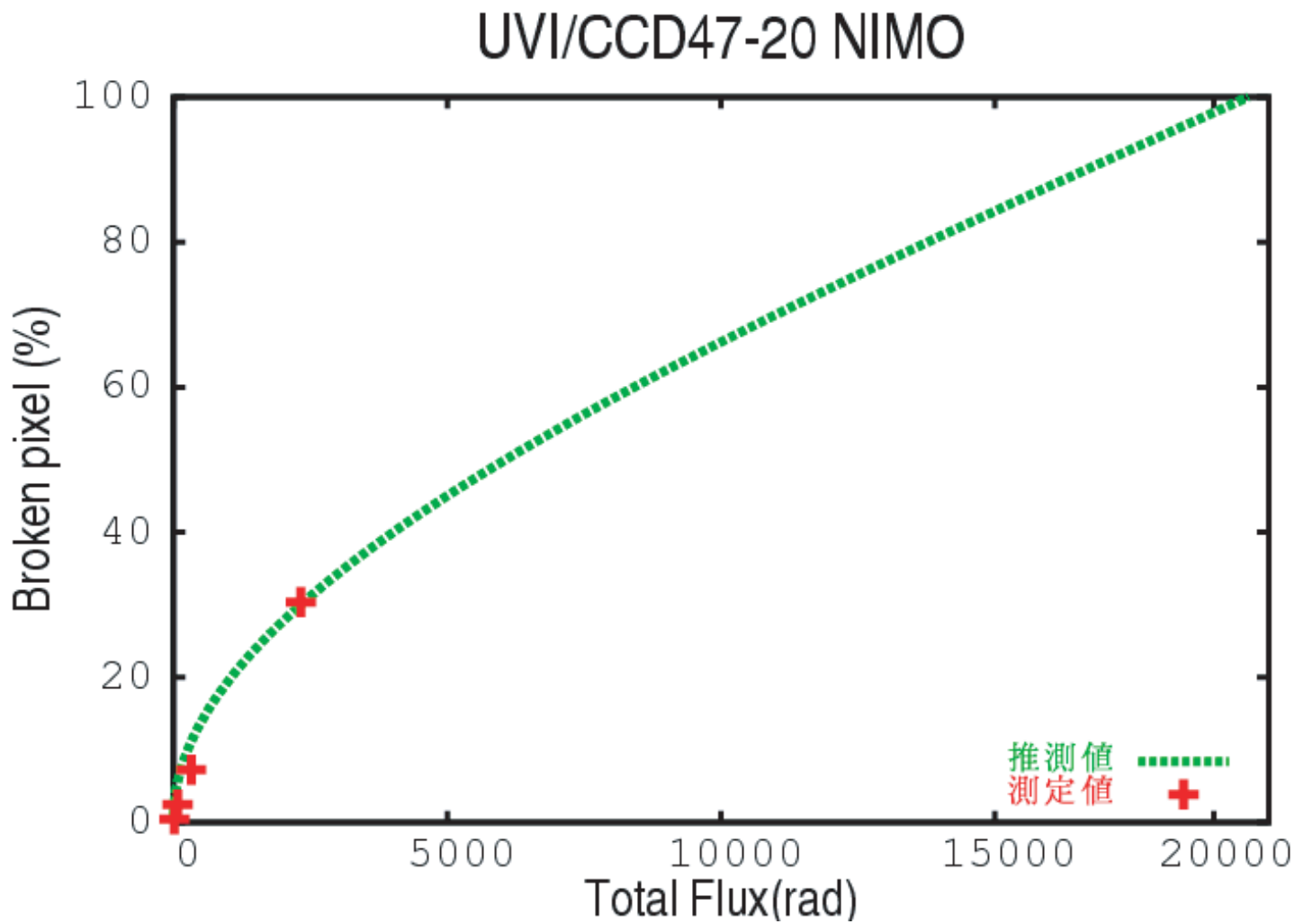
Fig.5.2: Relation between total dose and dark spikes of CCD47-20 NIMO. The presumed curve is estimated by probability calculation, and fitted with experiment values. Under 10 krad(s) total dose, it is expected that the half pixel of CCD receive some damages..
