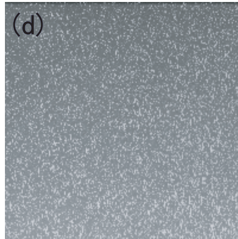
Fig.5.1: A part of CCD dark image (50x50 pixels) after 100MeV proton irradiation at several situation. As the amount of irradiation increases, the number of dark spike also increases. Each estimated total dose: (a): 12.8, (b): 72.8, (c): 322.8, (d): 2332.8 rad.
