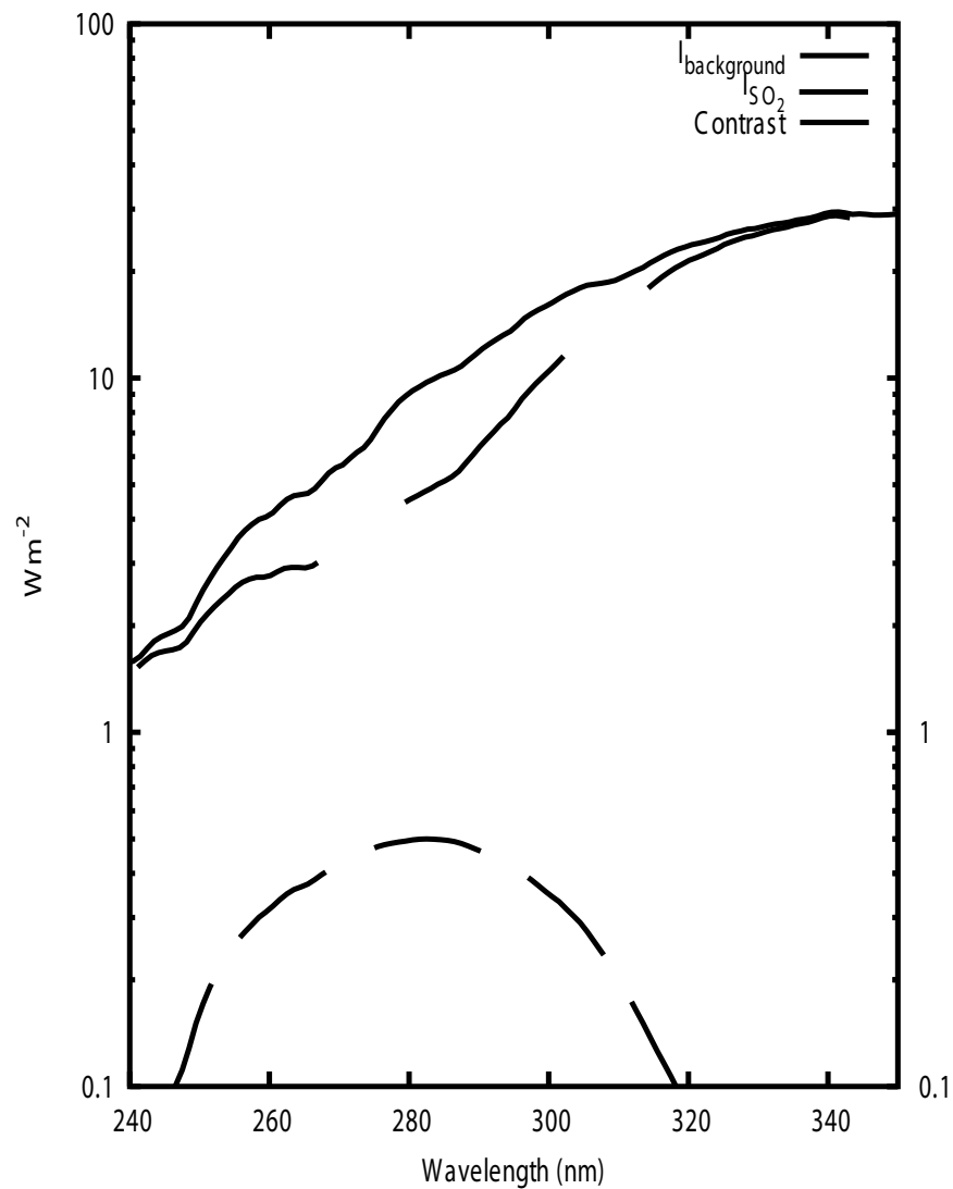
Fig.4.2: Presumption of the contrast by SO_2 absorption. The result about the case of dl=15nm . It becomes the contrast maximum when it is made the main wavelength of 282nm. The contrast maximum approaches 284nm of an absorption belt peak as dl becomes small.
