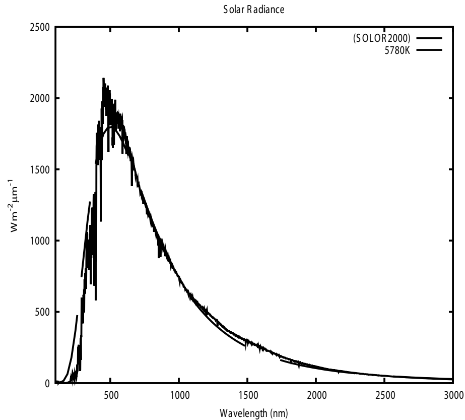
Fig.4.1: Spectrum of SOLAR2000 model and 5780K black body radiation in the Venus distance. Since solar radiation spectrum has the gap from that of black body radiation around ultra violet, the estimation is achieved using both 5780K black body radiation and SOLAR2000 model.
