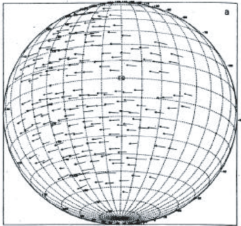
UV FEATURE MOTIONS..MARINER 10 OBSERVATIONS
